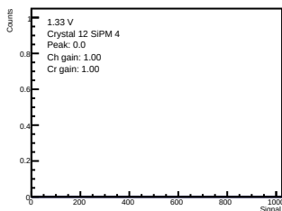
ADC-only | 1.33 V | crystal 12 | sipm 4
