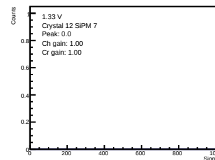
ADC-only | 1.33 V | crystal 12 | sipm 7
