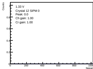
ADC-only | 1.33 V | crystal 12 | sipm 0
