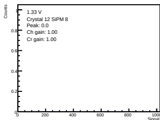
ADC-only | 1.33 V | crystal 12 | sipm 8
