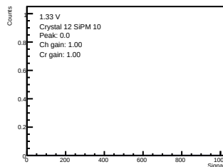
ADC-only | 1.33 V | crystal 12 | sipm 10
