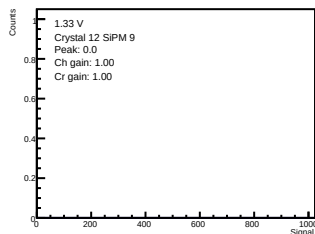
ADC-only | 1.33 V | crystal 12 | sipm 9
