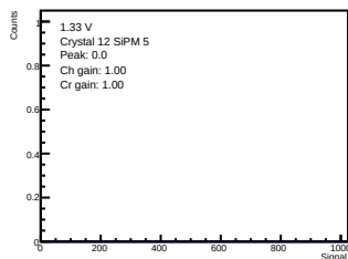
ADC-only | 1.33 V | crystal 12 | sipm 5
