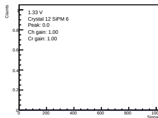
ADC-only | 1.33 V | crystal 12 | sipm 6
