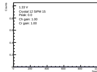
ADC-only | 1.33 V | crystal 12 | sipm 15
