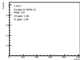
ADC-only | 1.33 V | crystal 12 | sipm 13
