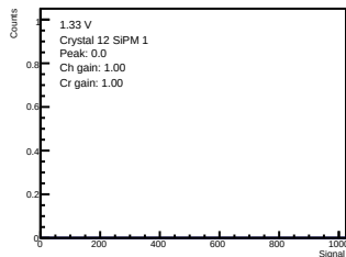
ADC-only | 1.33 V | crystal 12 | sipm 1
