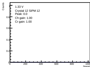
ADC-only | 1.33 V | crystal 12 | sipm 12
